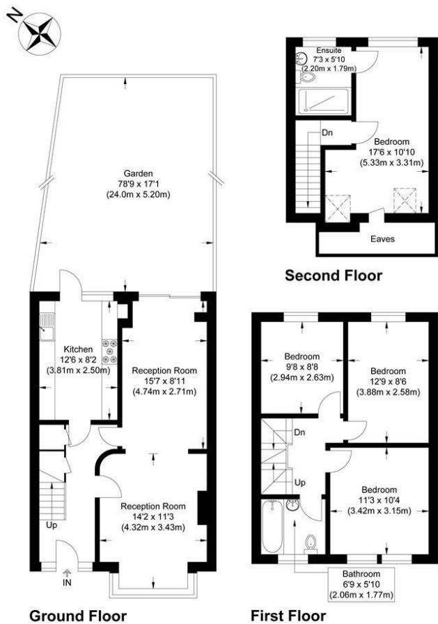
Cecil Avenue Approximate Gross Internal Floor Area : 109.5 sq m / 1178.64 sq ft. Illustration for identification purposes only, measurements are approximate, not to scale.
