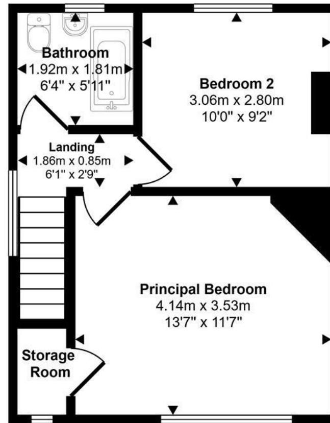
First Floor Approx 33 sq m / 356 sq ft
