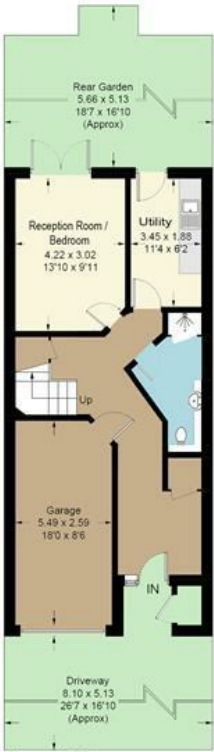
Ground Floor
