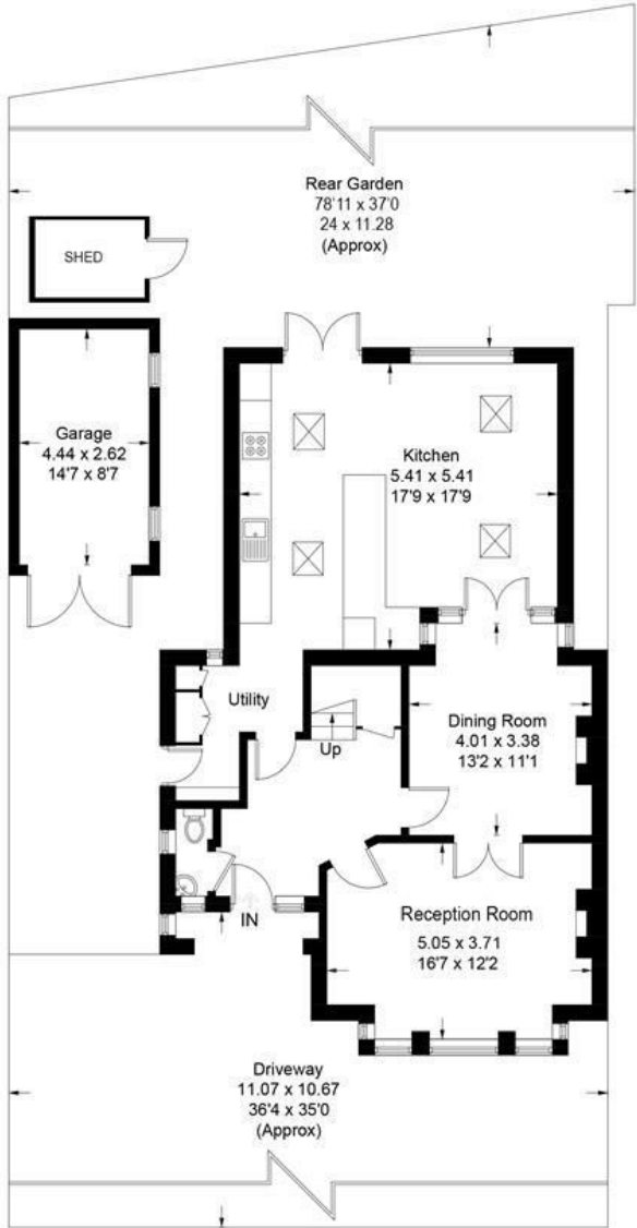
Ground Floor
