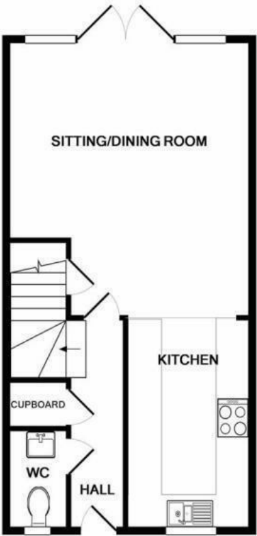
GROUND FLOOR APPROX. FLOOR AREA 451 SQ.FT. (41.9 SQ.M.)
