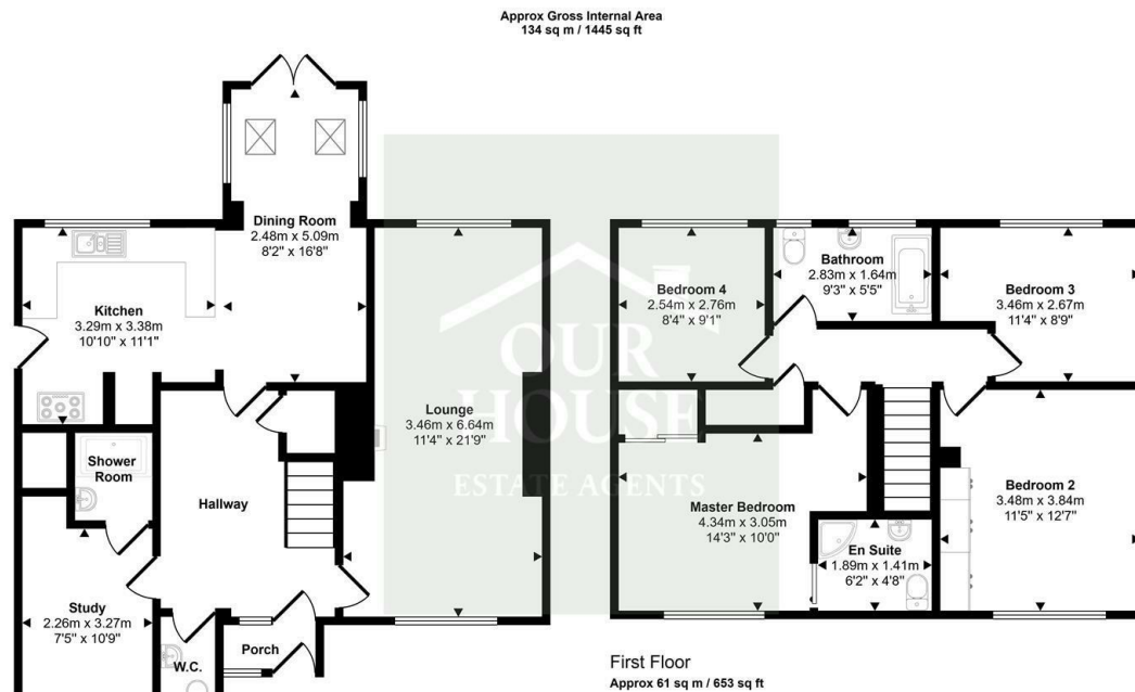
Ground Floor Approx 73 sq m / 791 sq ft
