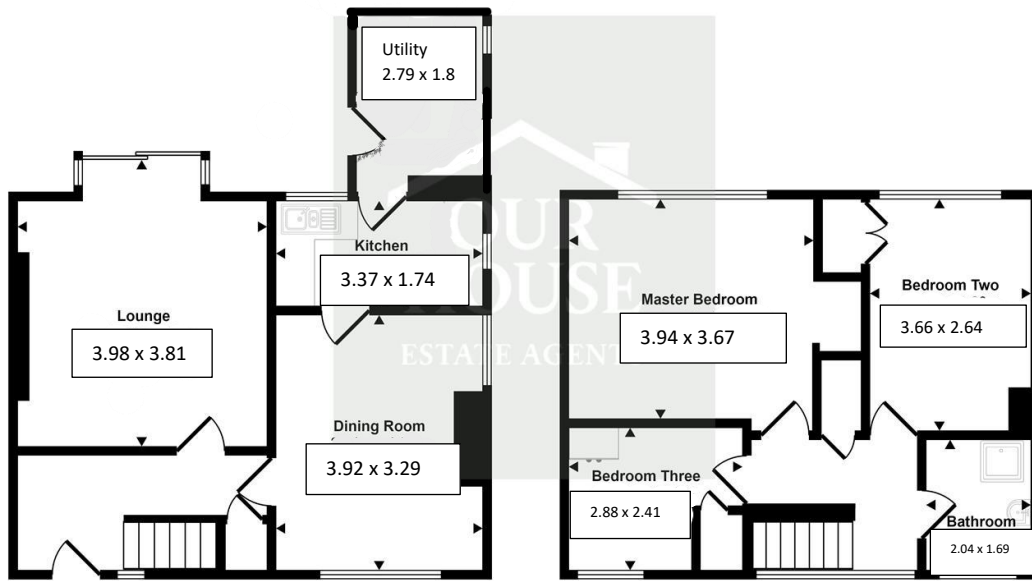
Ground Floor Approx 49 sq m / 529 sq ft
