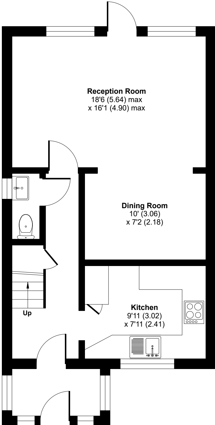
GROUND FLOOR
