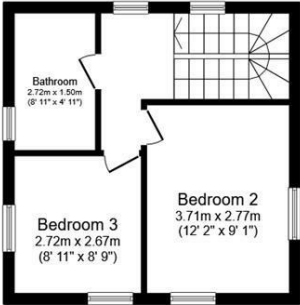
Second Floor Floor area 29.0 sq.m. (312 sq.ft.)
