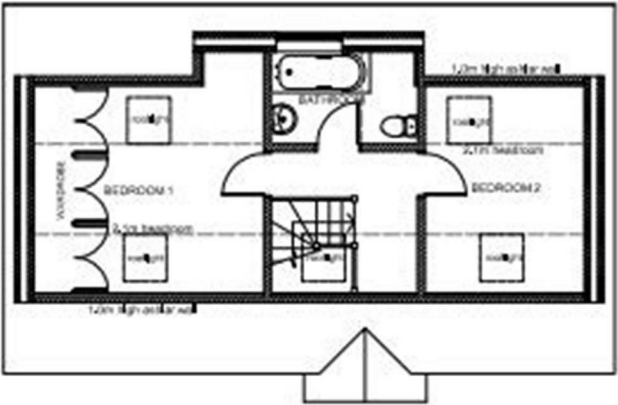
PROPOSED FIRST FLOOR PLAN 1:100
