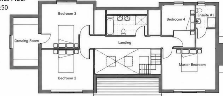
First Floor 1:50
