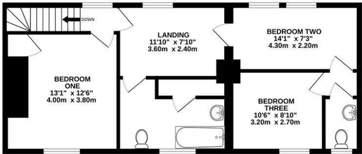
1ST FLOOR 596 sq.ft. (55.3 sq.m.) approx.
