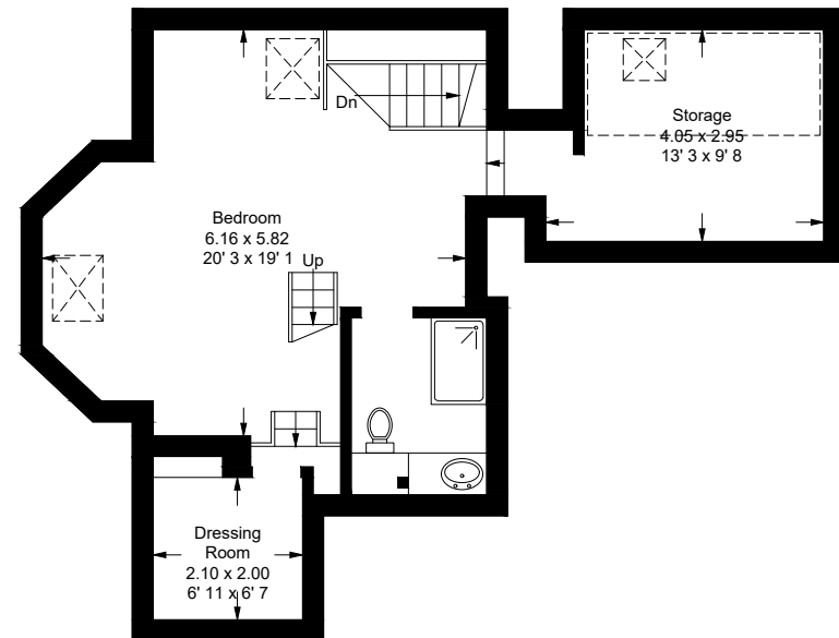
Second Floor 565 sq ft / 52.5 sq m (Including Reduced Headroom)
