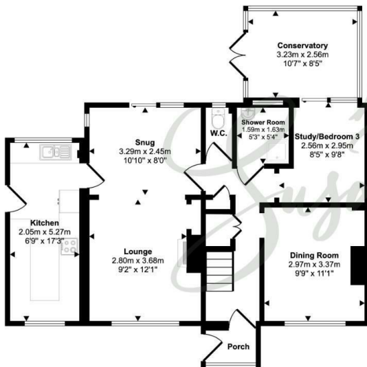
Ground Floor Approx 74 sq m / 800 sq ft
